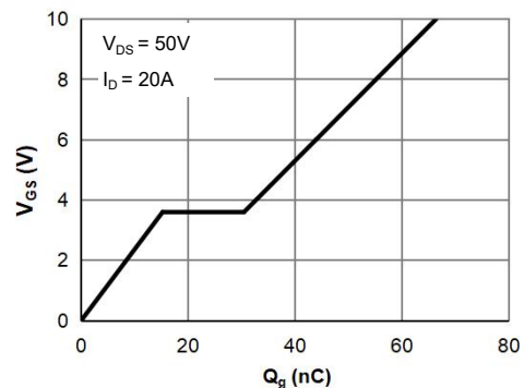
Gate Charge
